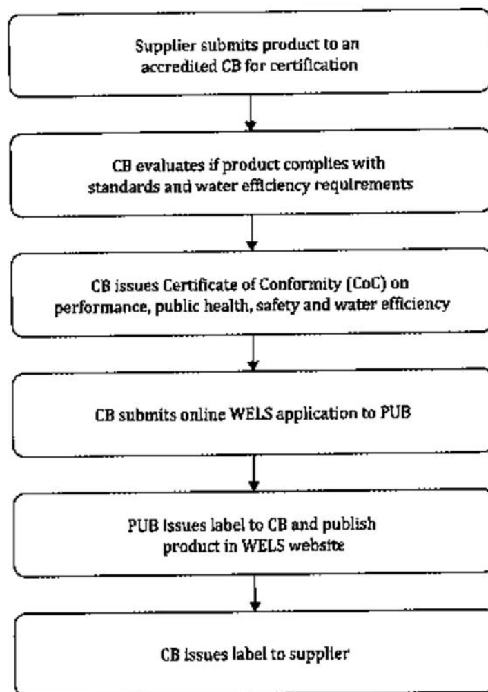
Figure D — 4 — Registration procedures of Singapore Water Efficiency Labelling Programme
