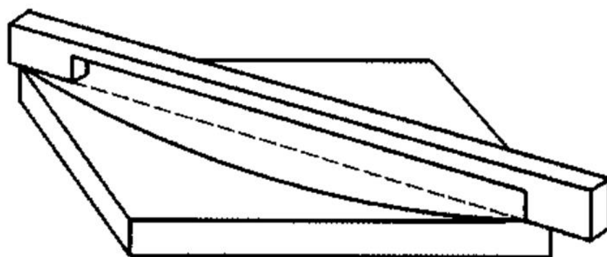
Figure 2 — Measurement of upper face flatness
