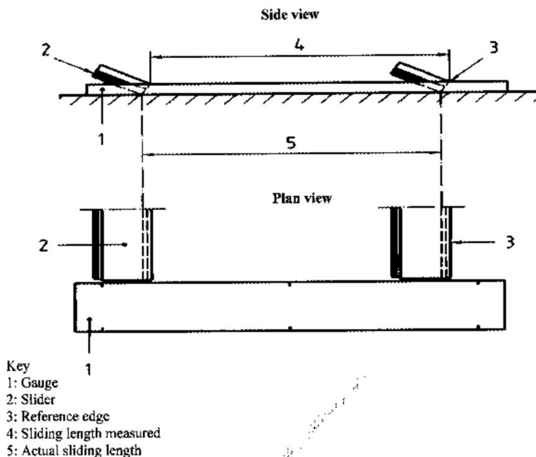
Figure 10 — Sliding length gauge
