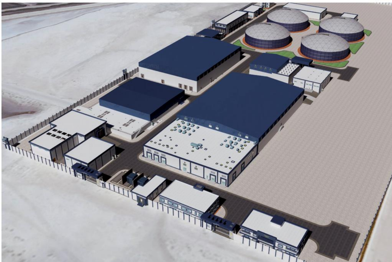
East Port Said SWRO Desalination Plant – 3D Layout: Detailed aerial view of the plant showing the arrangement of major process, utility, and support facilities within the site. The layout brings together the main treatment buildings, product water infrastructure, storage facilities, and operational buildings, with the site planned to support a desalination capacity of 150,000 m 3 /day, expandable to 250,000 m 3 /day. © ECG; Dorsch Global
